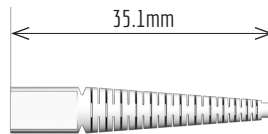
F4M-BTSC9P-X 900um Smooth Fiber Short SC Boot
